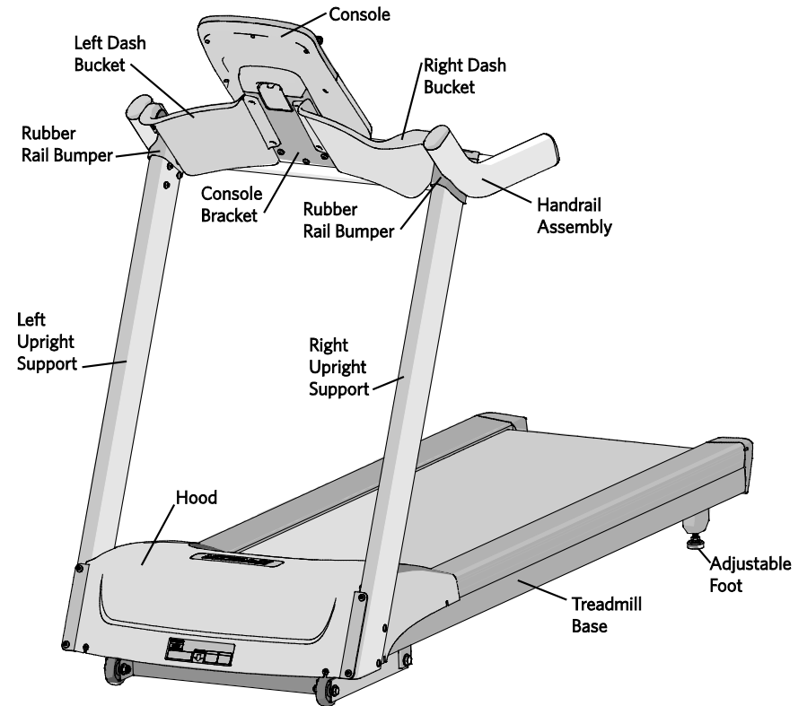
Figure 2: Major components of treadmill
