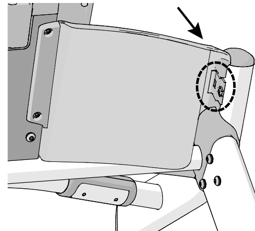
Figure 17: Dash bucket attachment
