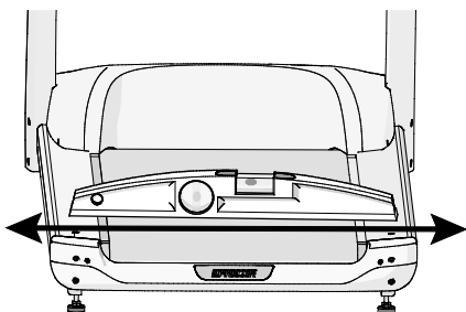
Figure 20: Level position across belt
