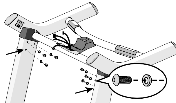
Figure 9: Handrail attachment and location of bottom hole
