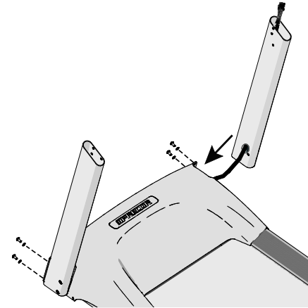
Figure 5: Base support front fasteners
