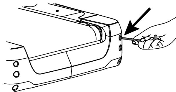
Figure 24: Belt adjustment bolt location
