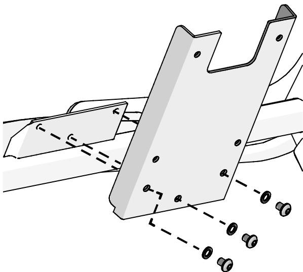
Figure 10: Console bracket attachment
